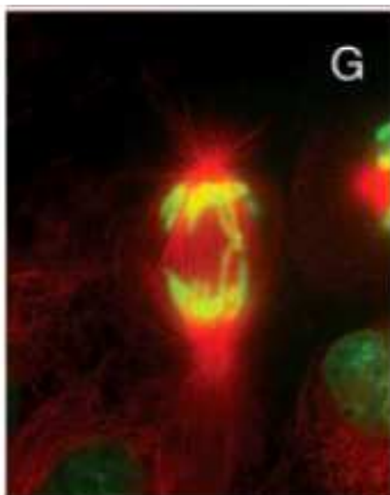
ANAPHASE
