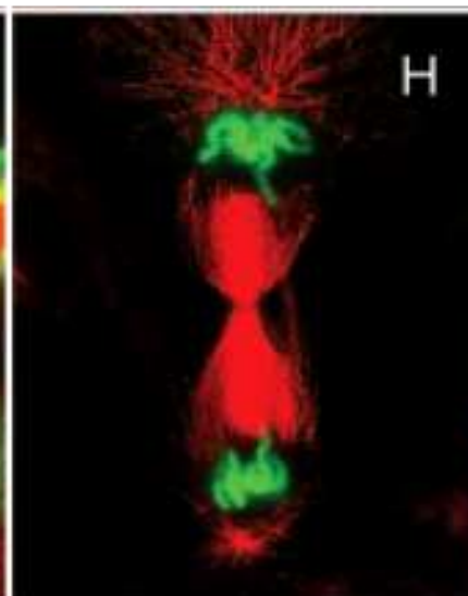
TELOPHASE
